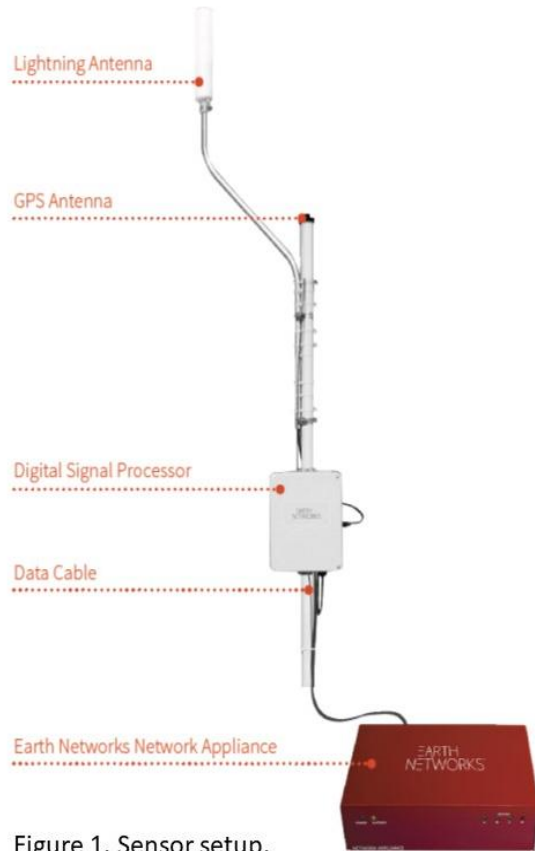
Figure 1. Sensor setup.
